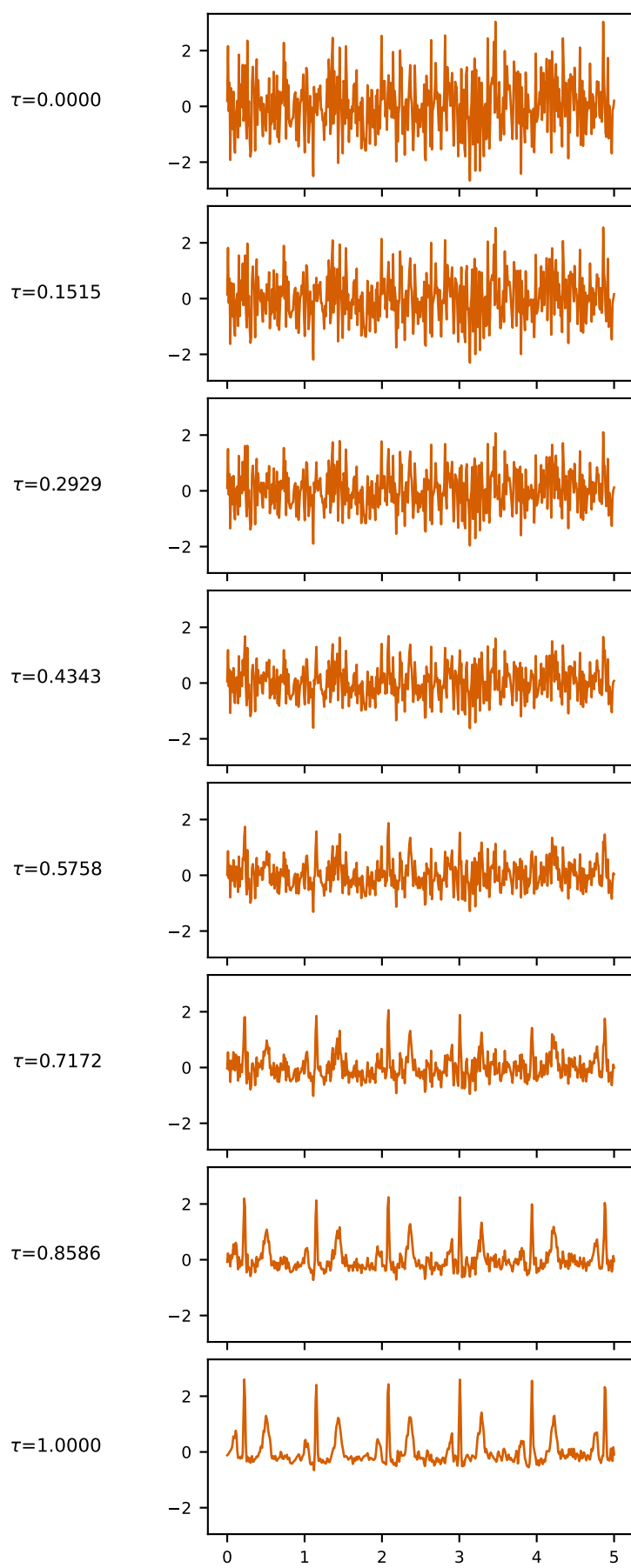
Flow matching
